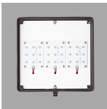
KT-WP12-27LED
